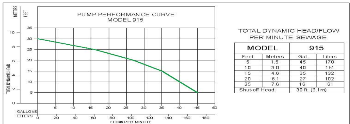
Performance curve 915 grinder system
